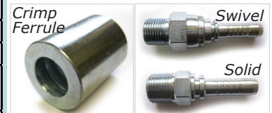
3/8" MPT x M swivel
